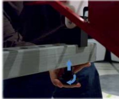
Non-stinger method to mount Model 3142E to 7-TR
