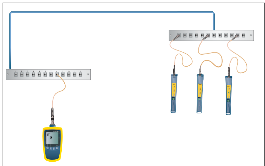
Figure 1. Using FindFiber mode to locate fibers – patch panel to wall outlet
