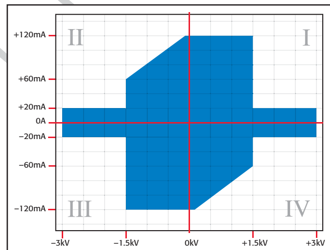
The Model 2657A can source or sink up to 3000V @ 20mA or 1500V @ 120mA.
