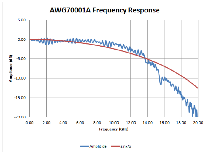
AWG70001A frequency response including Sin x/x
