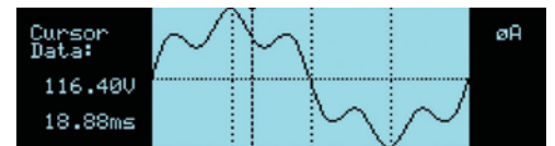
Acquired Voltage waveform (MX22.5/30/45 Display).
