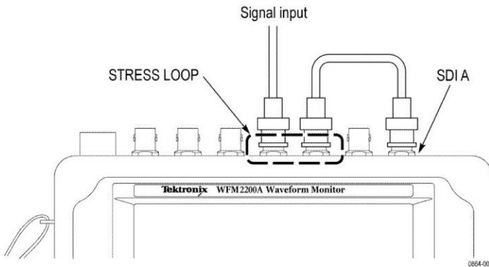
Stress loop connections for a monitored signal.
