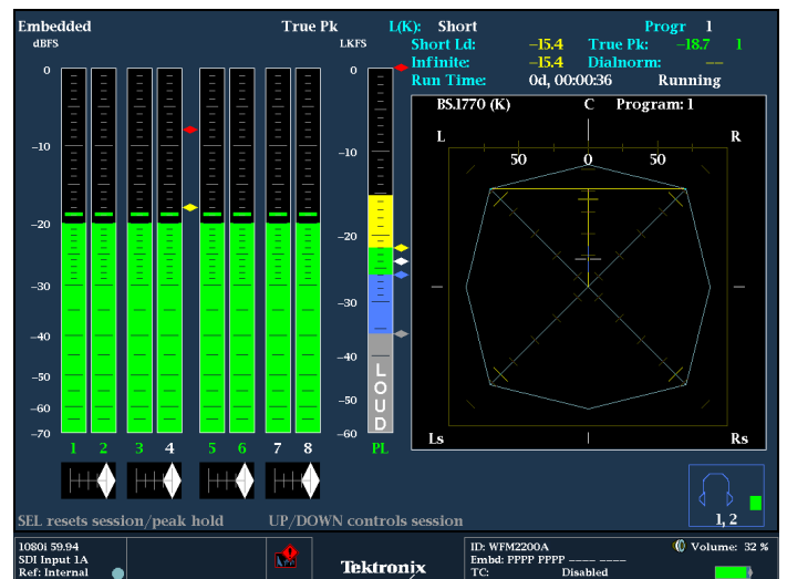
Audio display with Surround Sound monitoring.
