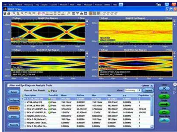
DPOJET PCE3 base specification measurement suite
